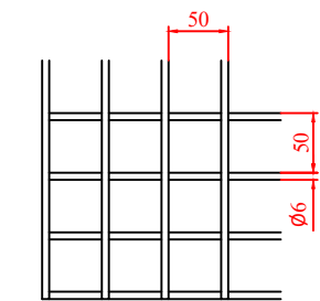
Treillis galva 1350x2750, fil Ø 6mm, maillage 50x50 G0105200
